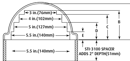
ALL MODELS END VIEW
