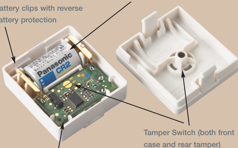
PCB with MEMS accelerometer chip
